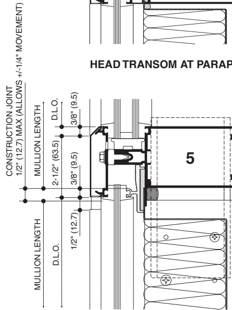
EXPANSION JOINT
