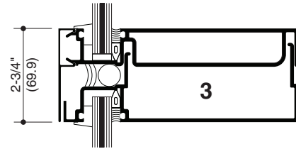
EXPANSION HORIZONTAL
